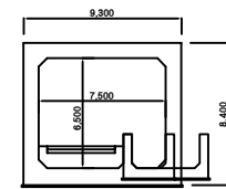
SECTION
